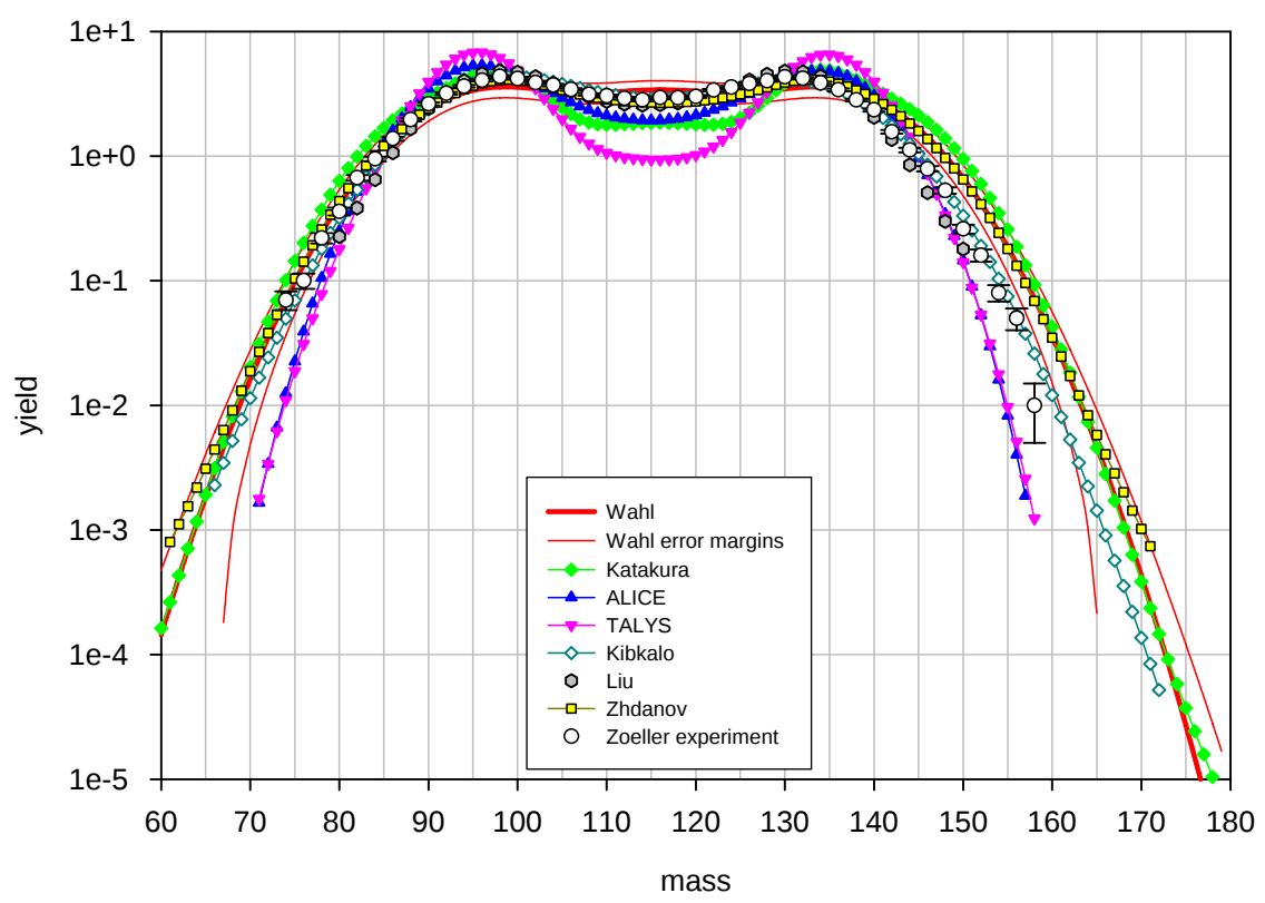
Benchmark A: ^{238}\text{U} at 50 MeV, post neutron emission yields
